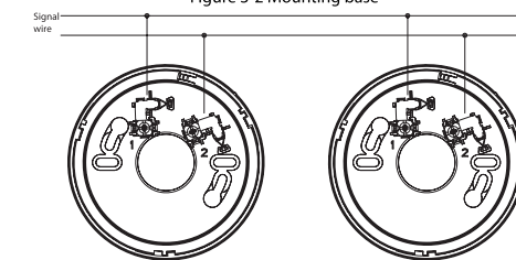
Figure 3-3 Installation (2)
