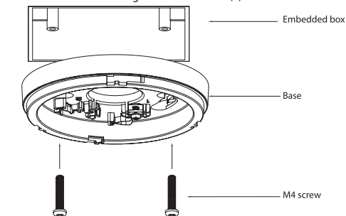
Figure 3-1 Installation (1)
